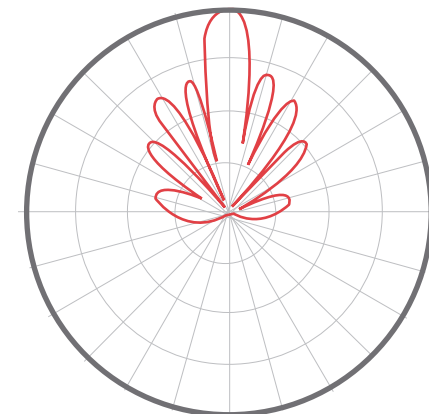
Elevation Radiation Pattern
